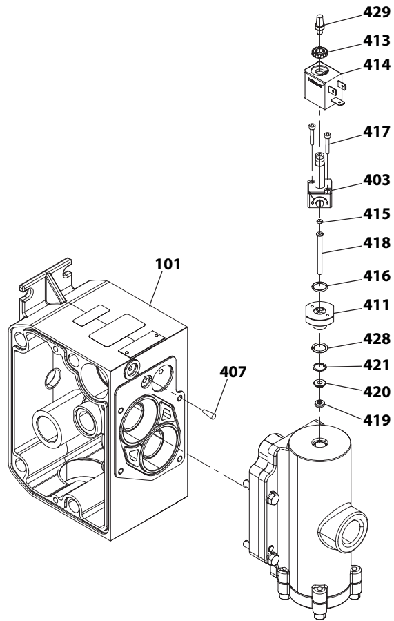
仅用于SD30S-XXX-XXX-AXX 型号
